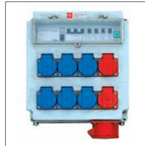
Electrical panel OCTANORM EUR 120.00 Code 019.010.275.000
